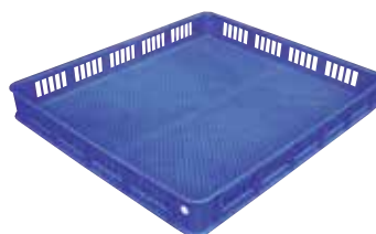
F658 曬乾籃(3) O.D.:635x556x81mm I.D.:616x537x69mm BOTTOM I.D.:610x530x60mm CAPACITY:19L
