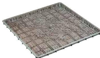
F991 曬乾籃(1) O.D.:948x948x56mm I.D.:909x909x43mm BOTTOM I.D.:870x872x32mm CAPACITY:32L 1578pcs/40ft'
